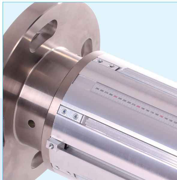
i2 Air Shaft.
